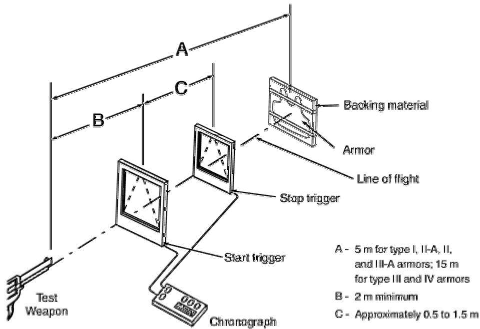
FIGURE 2. Ballistic Test Setup
